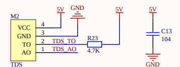
TDS传感器模块
